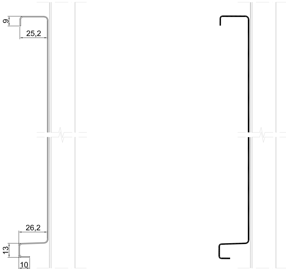
STANDING SEAM PROFILED TRAY
