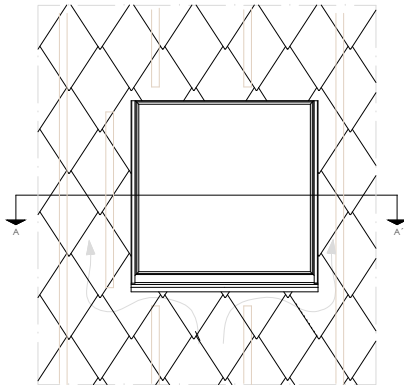
T D 7.2.02 Horizontal window section (Non-vented sill).
