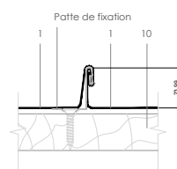
B. JOINT DEBOUT DOUBLE SERTISSAGE
