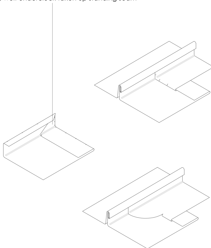
Cross welt underclock taken up standing seam
