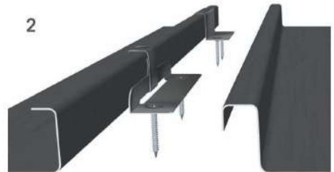
Clipped undercloak and the overcloak
