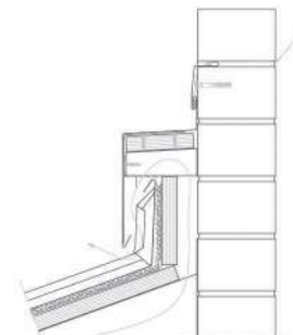
Vented abutment to brick wall
