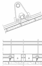
Double pipe system with ice breaker
