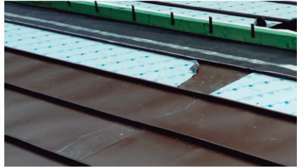
Partial removal of protective film causing marking of Rainbow brown – this can be wiped away.
